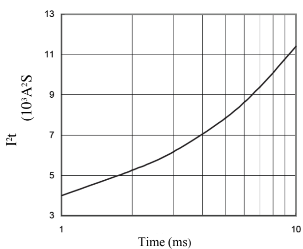
I^2t Characteristics
